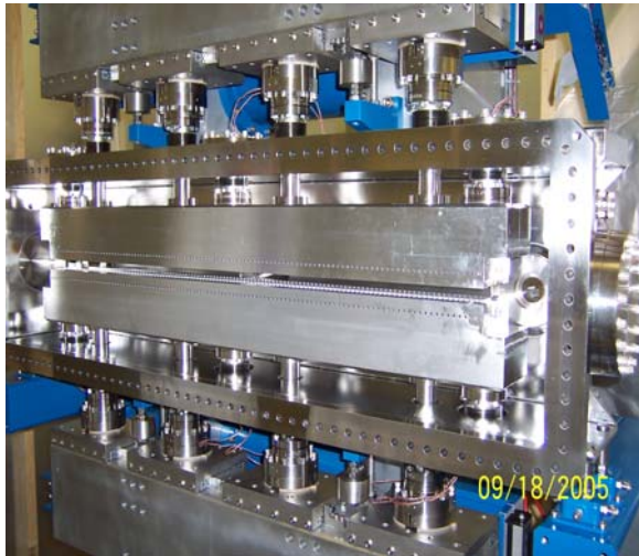
Figure 7. The fully opened jaw (19 mm) at chamber can ease the magnet for measurement and shimming
