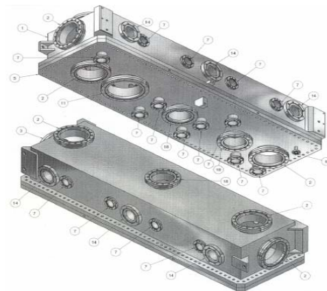
Figure 6. Chamber drawing shows a full-size removable front panel and multi build-in ports
