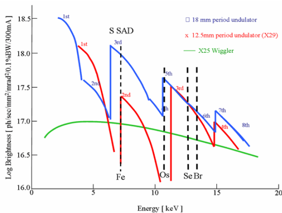
Figure 9. The harmonics and periods of undulator and wiggler are shown in the brightness vs. energy plot
